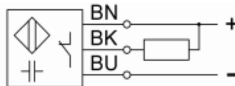
Wiring Diagram
