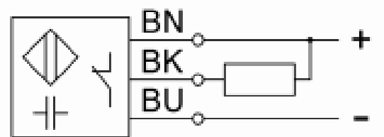
Wiring Diagram
