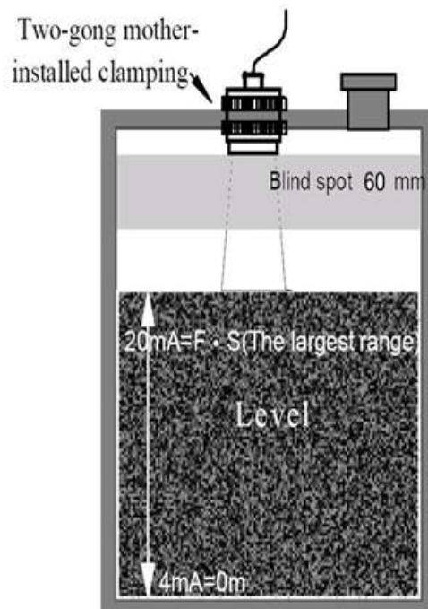
UE3005 Ultrasonic Level Sensors Installation Example
