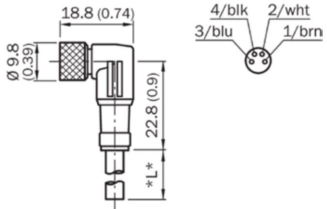
Connection diagram
